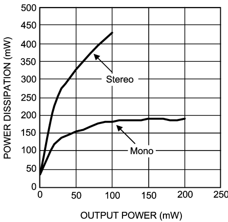
Power Dissipation vs Output Power V_{DD} = 3.6V, R_L = 16\Omega, f = 1kHz
